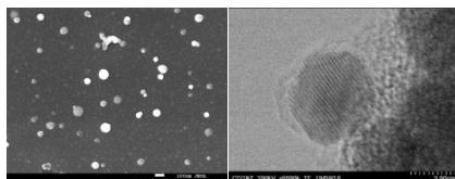
Fig. 1 a) SEM image of topography of C-Au film, b) UHR TEM image of C-Au film
