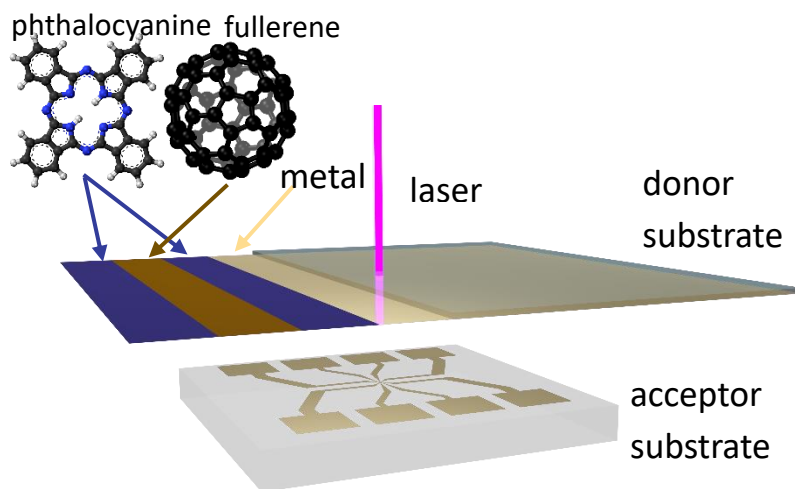
Fig. 1: CW-LIFT scheme
